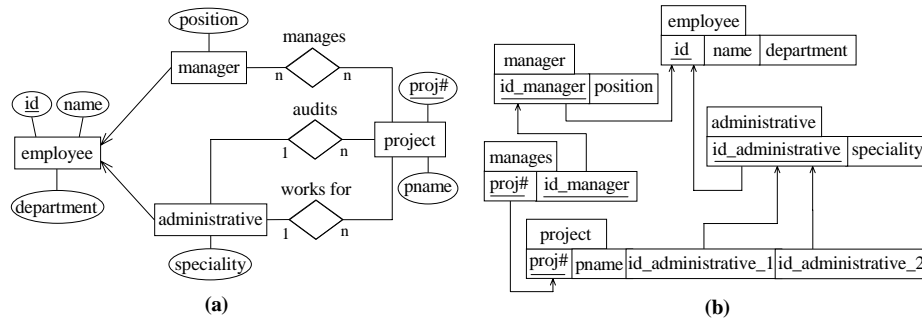
Fig. 2. Examples of Conceptual and Logical Database Schemas
