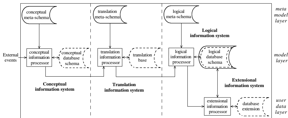
Fig. 4. Architecture for Database Evolution
