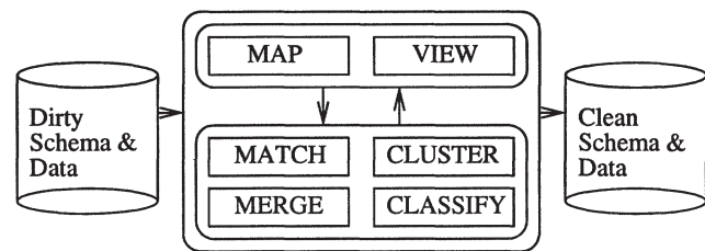
Figure 1: The BIO-AJAX framework.
