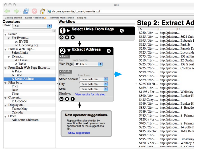
Figure 1. Marmite is an end-user programming tool for creating web-based mashups. On the left is a set of operators that users can select to extract and process data from web pages. In the middle is the data flow, and on the right is a spreadsheet view that shows the current values of the data.
